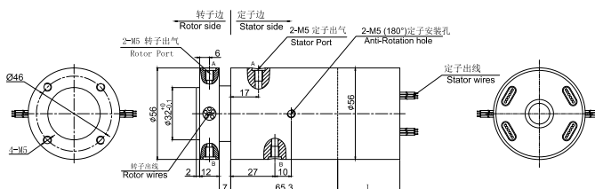
MAPH200F-01+Electricity size
